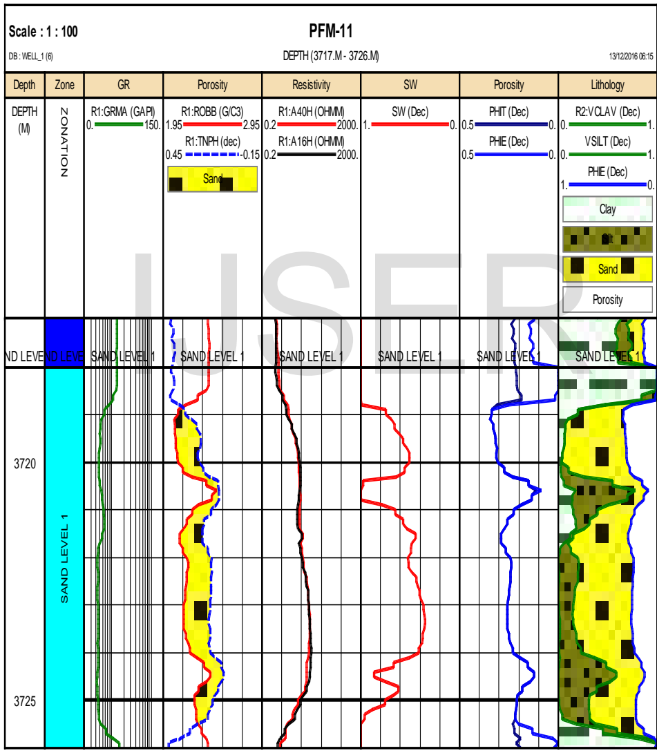
Fig. 10 Litho-Saturation Cross-Plot of PFM-11 Well
