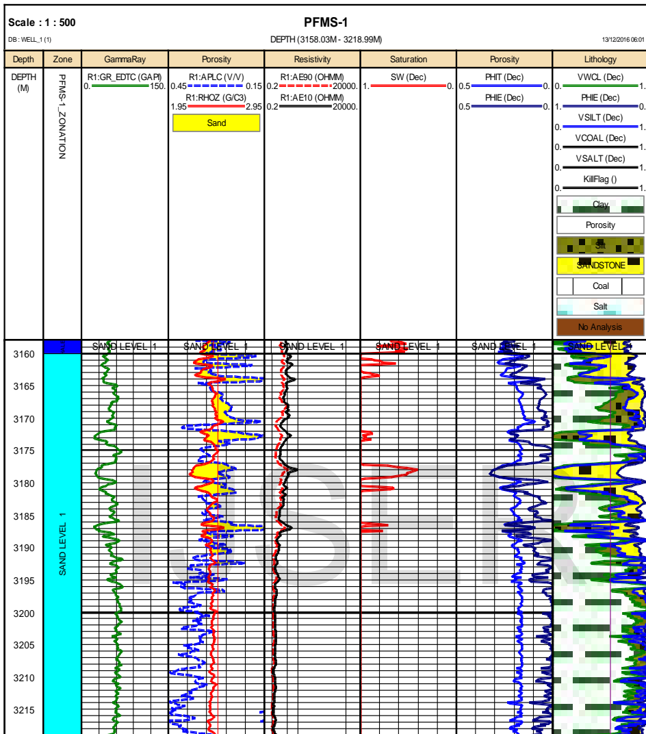
Fig. 6.Litho-SaturationCross-Plot of PFMS-1 Well (Wakar Fm. Sand Level-1).
