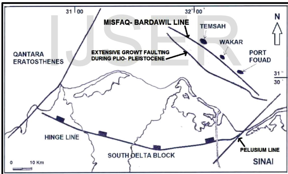
Fig. 4 Regional structural setting, north Nile Delta [12,5].
