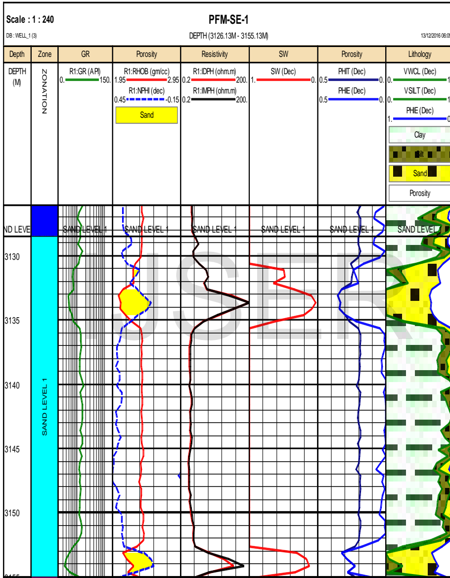
Fig. 8 Litho-Saturation Cross-Plot of PFM-SE-1 Well
