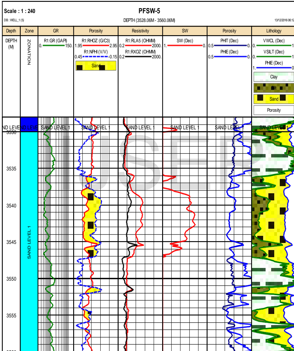
Fig. 9 Litho-Saturation Cross-Plot of PFM-SW-5 Well
