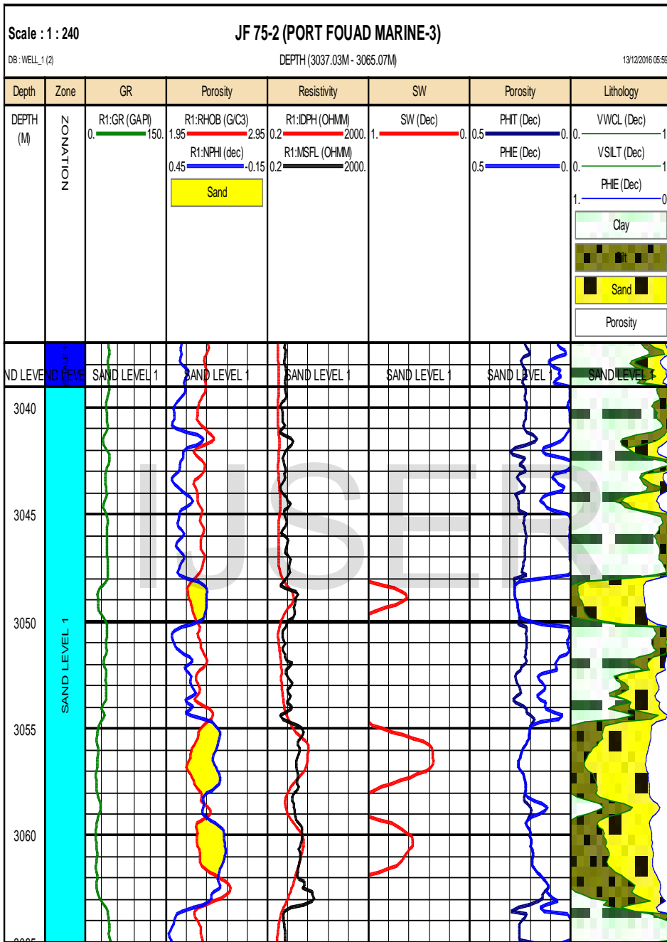
Fig. 7 Litho-Saturation Cross-Plot of PFM-3 Well
